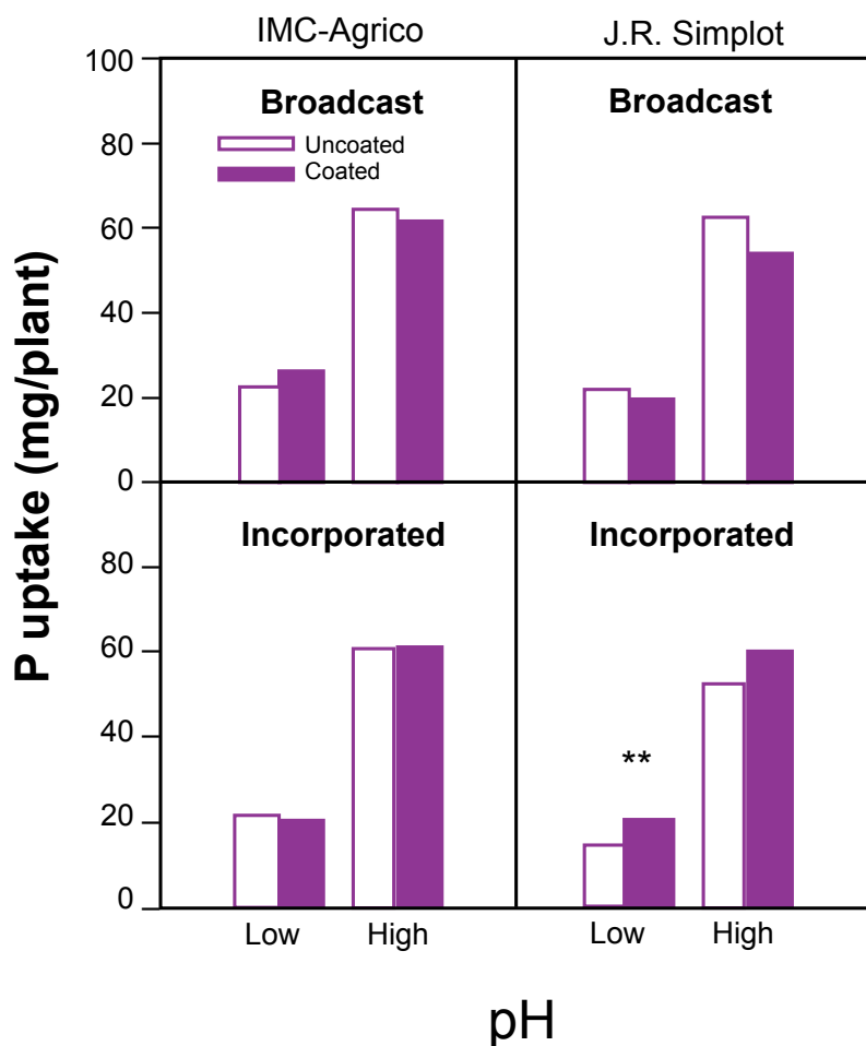
Figure 4. Effects of coatings on P uptake in corn from two MAP fertilizer manufacturers. Initial Olsen P = 10 ppm and 12 ppm for low and high pH soils, respectively (Jones and Jacobsen, 2005). ** - significant at P < 0.05
