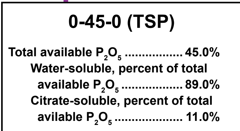
Figure 7. Example of the water-soluble P content and citrate-soluble P content for TSP.
